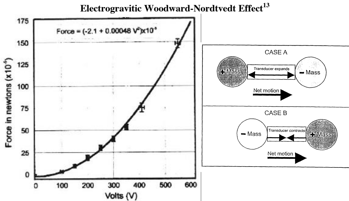
FIGURE 1. Force ( 10^{-5} N = dynes) Output Vs. Capacitor Voltage (V) Input of a Woodward Force Transducer (Mahood, 2000) and the Net Motion Direction of Cases A and B (Woodward, 2000).
